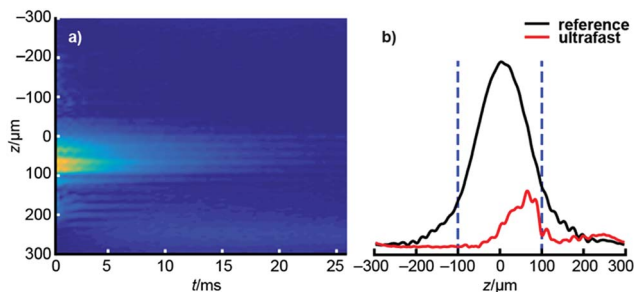
Fig. 2 (a) The raw data of the ultrafast D - T_2 experiment of hyperpolarized water. The vertical axis represents the spatial dimension, acquired following Fourier transform of each echo individually, while the horizontal axis represents the time at which each echo is acquired. The time projection (sum of all columns) is shown on the right. (b) Comparison of the signal profiles of the ultrafast (red) and reference (black) experiments. In the post processing, the ultrafast data was divided by the reference profile in order to eliminate the effect of inhomogeneous sensitivity of the rf coil across the sample. Dashed blue bars indicate the spatial bandwidth of the CHIRP pulse, 200 \mu\text{m} in this example.
