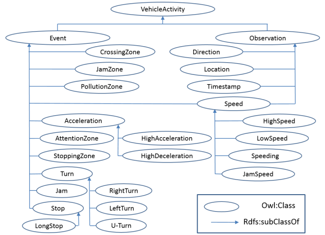
Fig. 1. High level static ontology for semantic reasoning in transportation system use case.
