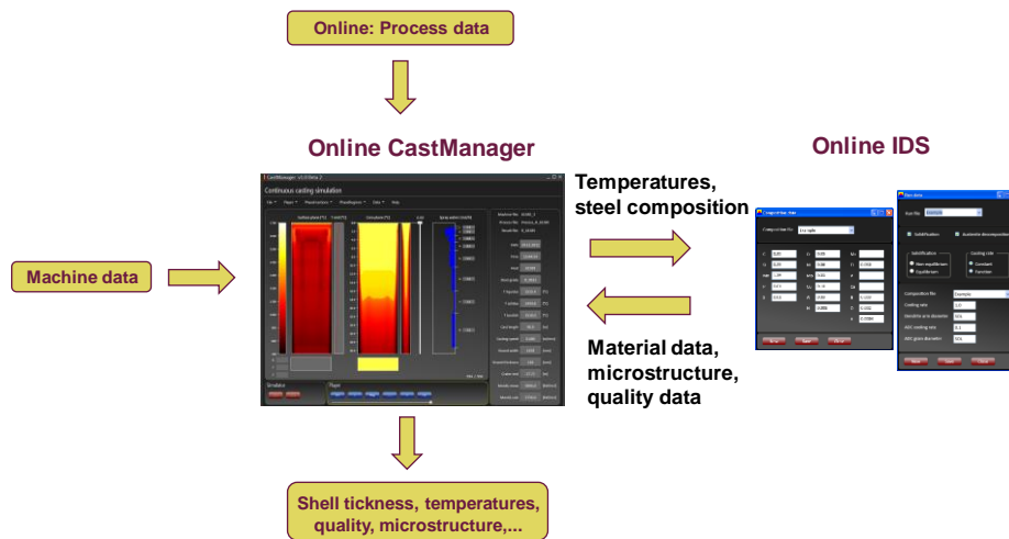
Figure 1. IDS and CastManager integrated online system for continuous casting.
