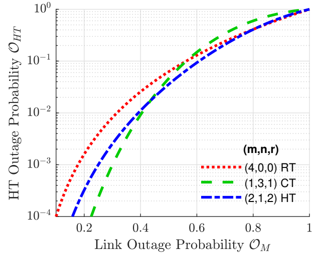
Figure 1. Final outage probability (after replication) versus link outage probability (before replication) for different HT configurations with M = 4 .
