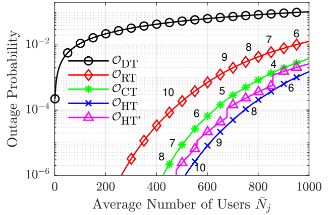
Figure 2. Outage probability of SF7 for each scheme using optimal configuration for different number of users \bar{N}_7 .
