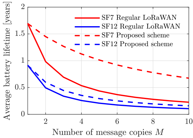
Figure 4. Average device lifetime using SF7 and SF12 for default LoRaWAN and the proposed modified protocol.
