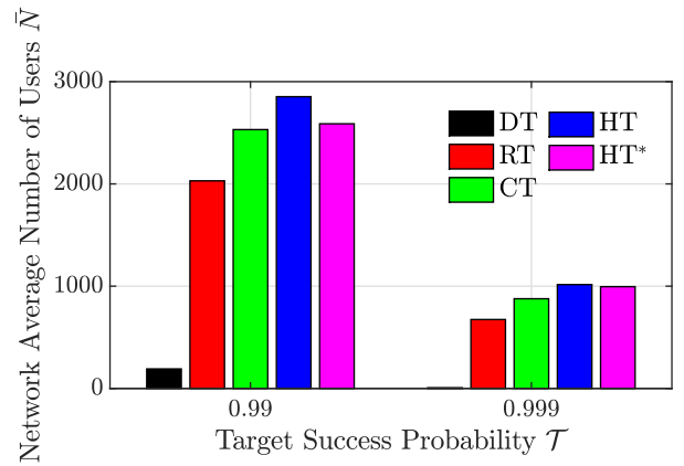
Figure 3. Average number of nodes \bar{N} for each scheme and reliability targets \mathcal{T} \in \{0.99, 0.999\} .
