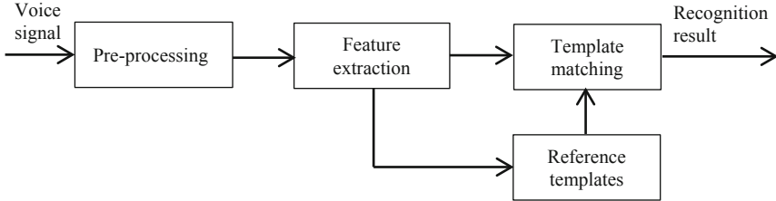
Fig. 2. Speech recognition system on a Sunplus MCU
