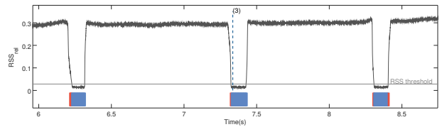
Figure 10. Positive detection by the threshold method.
