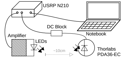
Figure 2. Measurement lab setup.
