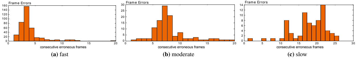
Figure 4. Histogram of frame error length (corrupt and missing frames combined).
