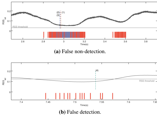
Figure 11. False decisions by the dwell timer (4).
