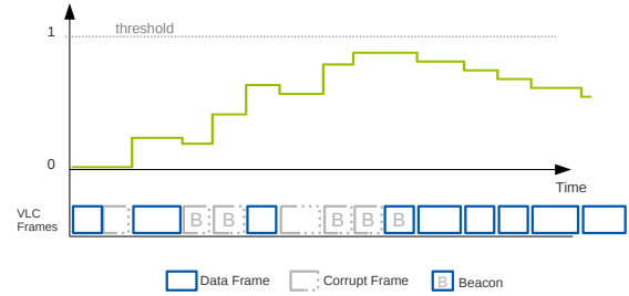
Figure 6. Example of a simple threshold decision algorithm.
