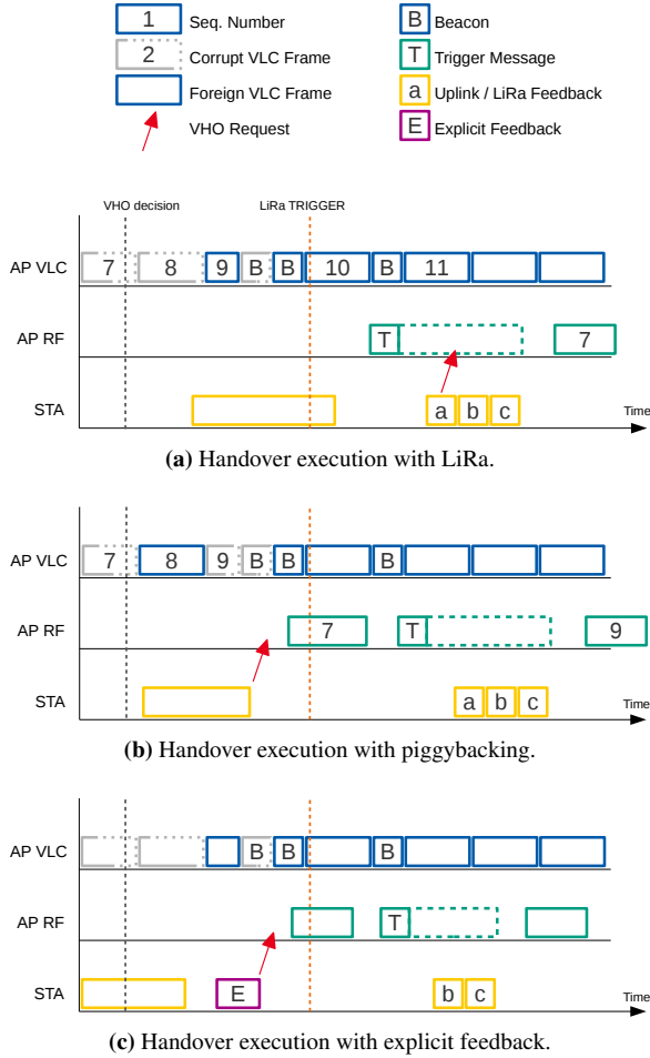
Figure 8. Station-based handover execution strategies.
