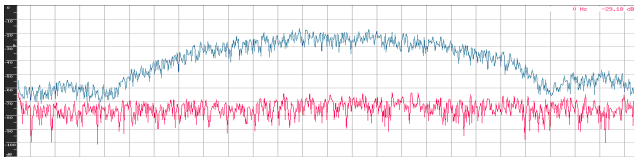
Figure 7. Frequency spectrum: signals (blue), noise (red).
