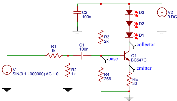
Figure 1. Schematic of our low-cost transmitter front-end.
