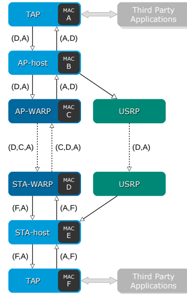
Figure 3. Flow of MAC layer frames. Wired connections: continues lines, wireless connections: dashed lines. Edge annotations: (destination, source) for Ethernet and VLC, (receiver, transmitter, destination) for WiFi.
