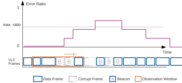
Figure 5. Simplified example of the error ratio method.
