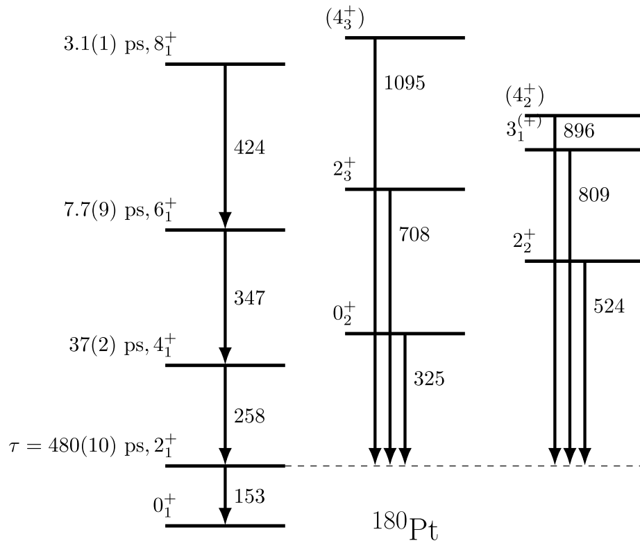
Fig. 3. A partial level scheme showing some of the low-lying states in ^{180}\text{Pt} [14]. The energies of a selection of the transitions feeding the yrast 2_1^+ state of interest are also shown in kilo-electron-volts, with measured lifetimes from taken from Ref. [19], with the exception of \tau_{2_1^+} , which was measured in the present work.
