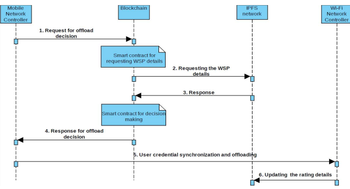
Fig. 3: Blockchain Sequence diagram
