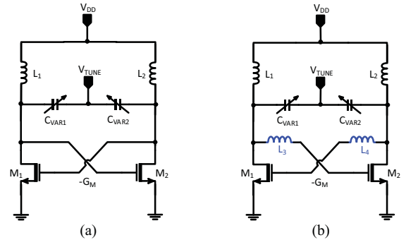
Fig. 1. (a) Conventional cross-coupled LC oscillator (b) An Inductive divider cross-coupled LC oscillator.
