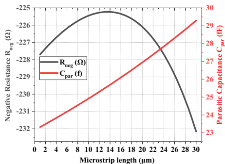
Fig. 8. At 130 GHz ( R_{neg} and C_{par} versus Transmission line length ( \mu\text{m} ))
