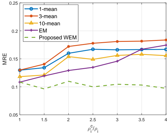
Fig. 5: MRE of the WEM approach and two baselines.
