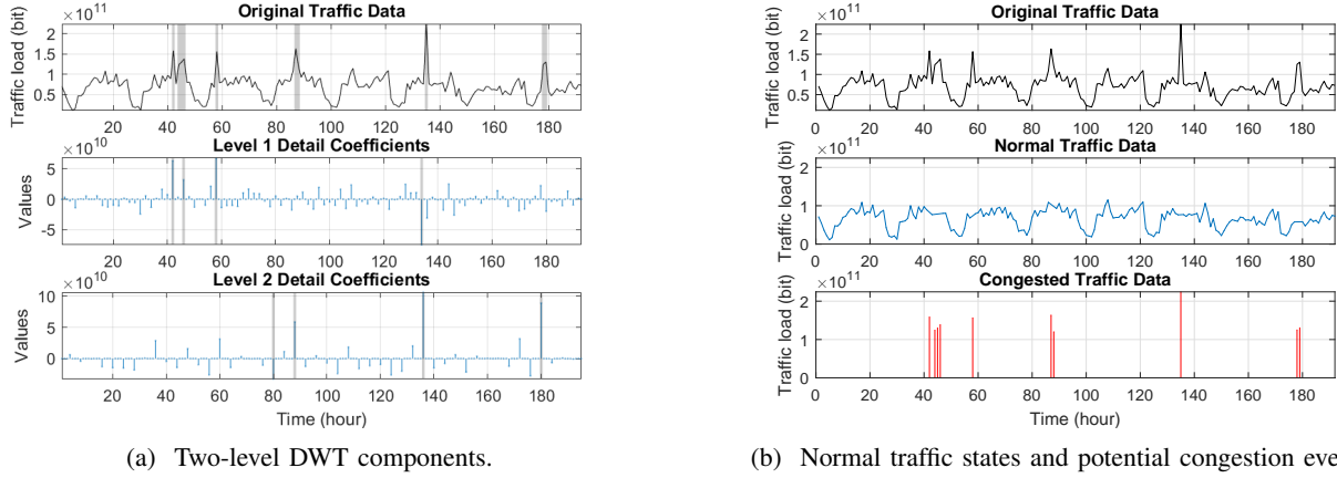
Fig. 3: Two-level DWT is applied to detect the cellular traffic congestion from a city level.
