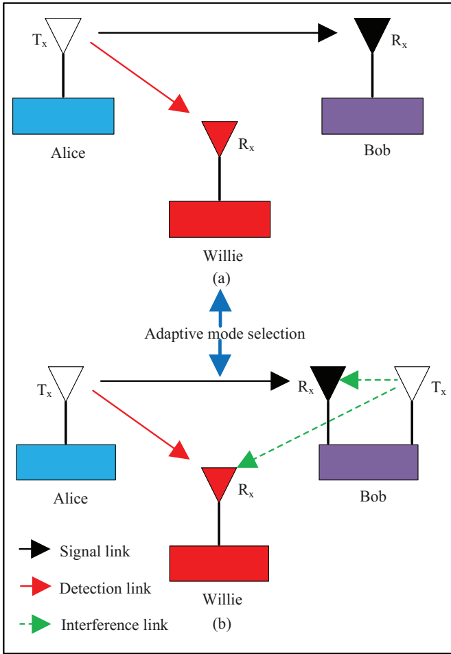
Fig. 3. Communication mode selection: a) Half-duplex mode; b) Full-duplex mode.
