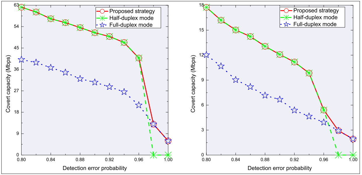
Fig. 5. Covert capacity in the scenario with UAVs as flying BSs: a) covert capacity of D2D link; b) covert capacity of cellular link.
