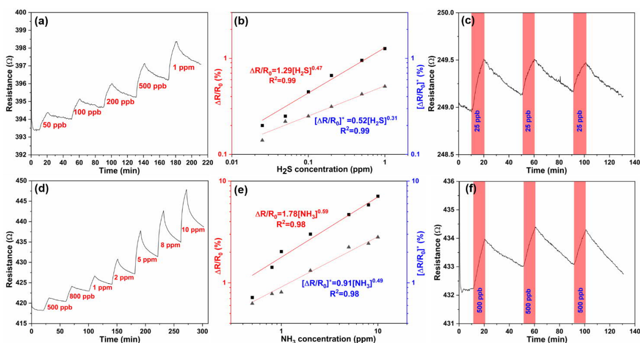
Figure 4 Transient gas response curves of PDNS-3 for the detection of (a) H 2 S from 50 ppb to 1 ppm, and (d) NH 3 from 500 ppb to 10 ppm with their corresponding plots of the responses and calibration curves in panels (b) and (e). Repeatability of response curves measured for (c) 25 ppb H 2 S and (f) 500 ppb NH 3 .
