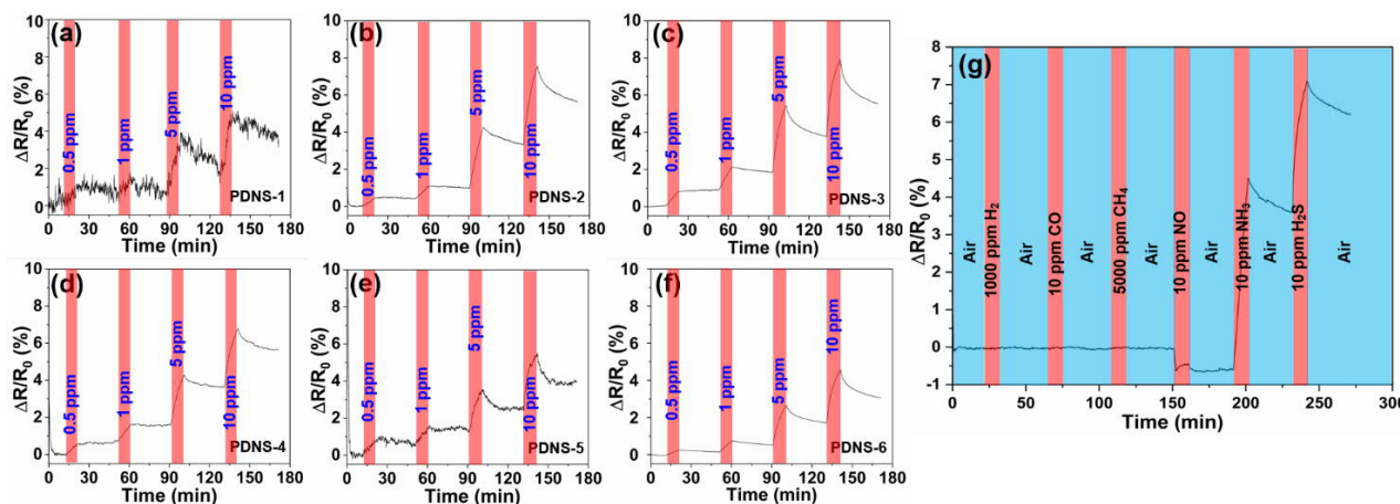
Figure 3 Transient responses curve of sensors based on PDNS-SWCNT composites with SWCNT concentrations of (a) 2 wt.%, (b) 5 wt.%, (c) 10 wt.%, (d) 20 wt.%, (e) 50 wt.% and (f) 70 wt.% measured for \text{NH}_3 at concentrations of 500 ppb, 1 ppm, 5 ppm, and 10 ppm. (g) Gas response of PDNS-3 composite (10 wt.% SWCNT) to various analytes in air buffer.
