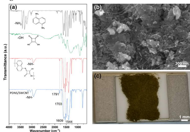
Figure 2 (a) FT-IR spectra of reactants, PDNS and the composite of PDNS/SWCNT. (b) SEM image of the
