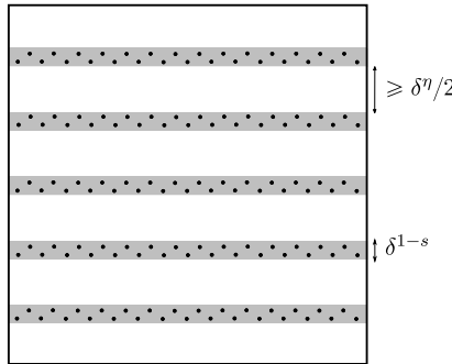
Fig. 2. The construction in Proposition 5.2.
